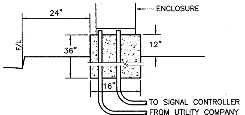
FOUNDATION PROFILE
