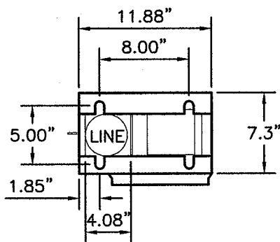
BASE PLAN
