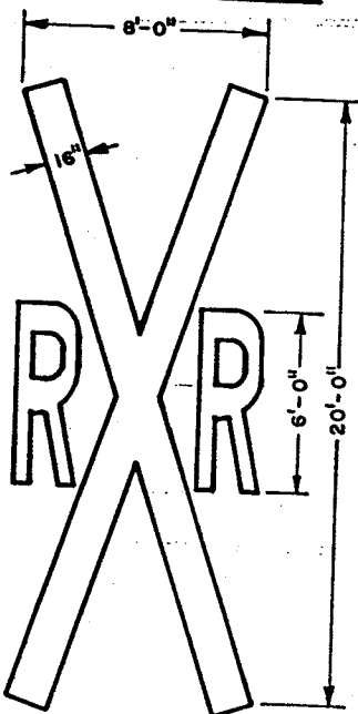
RAILROAD CROSSING SYMBOL
