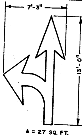
TYPE VII (L) ARROW (FOR TYPE VII (R) ARROW USE MIRROR IMAGE)
