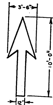
TYPE I (10) ARROW
