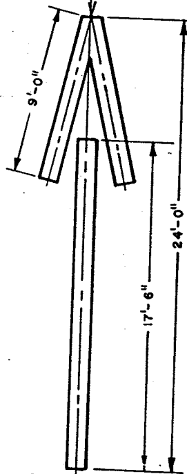
TYPE V ARROW
