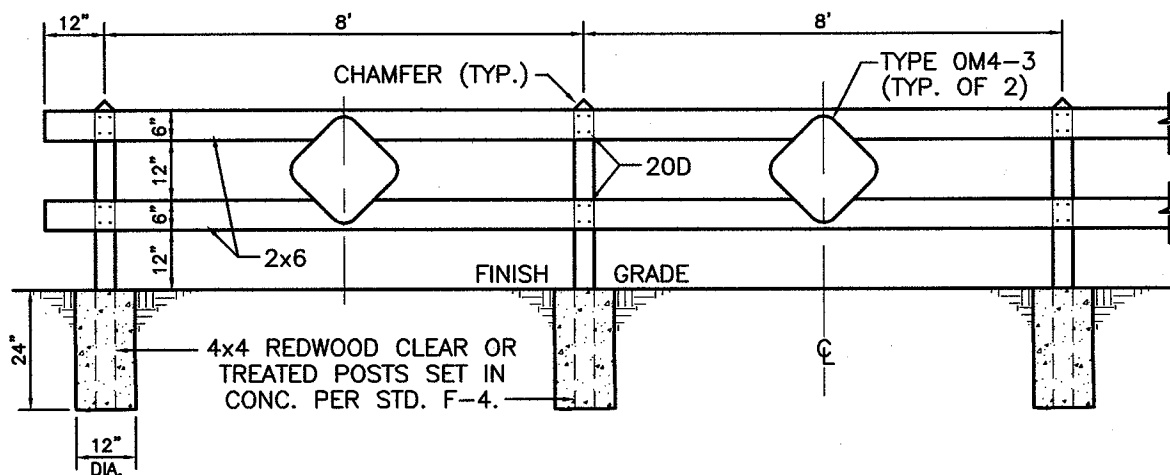
TYPICAL SIDE PANEL
