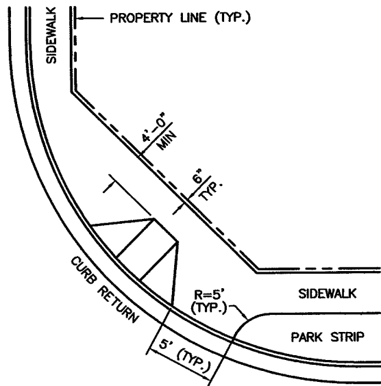
SIDEWALK TRANSITION FROM ADJACENT TO NOT ADJACENT
