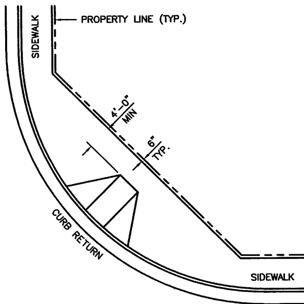
SIDEWALK ADJACENT TO CURB
