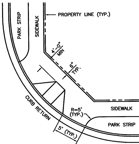
SIDEWALK WITH PARKSTRIP
