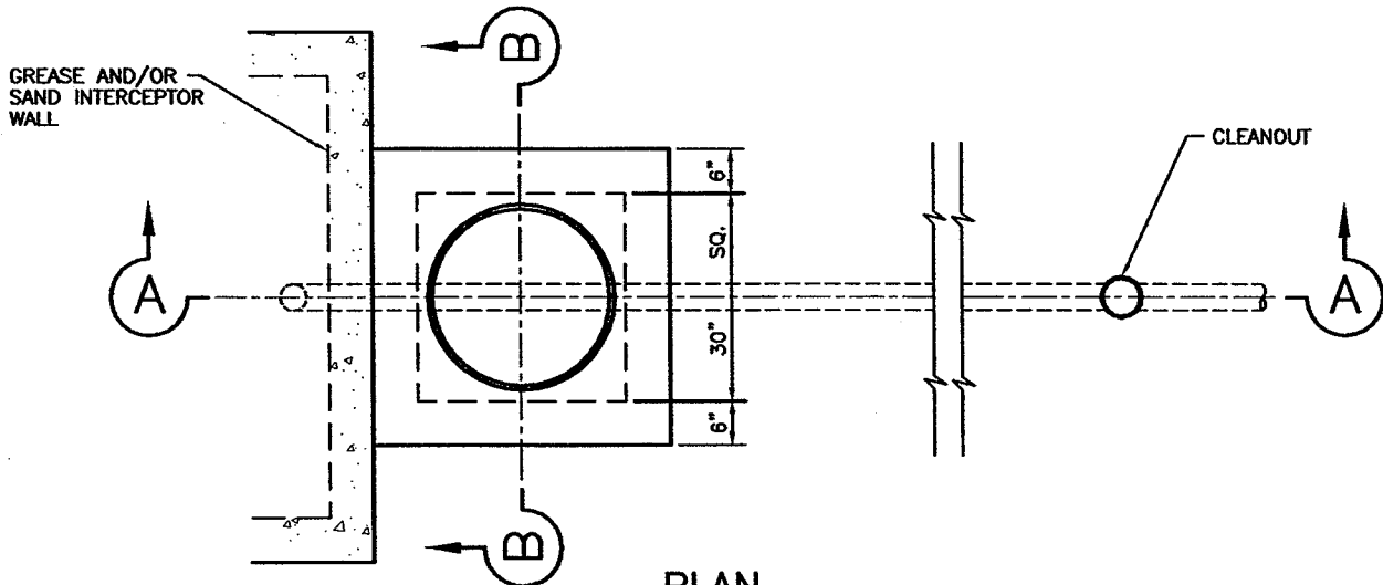
PLAN NTS
