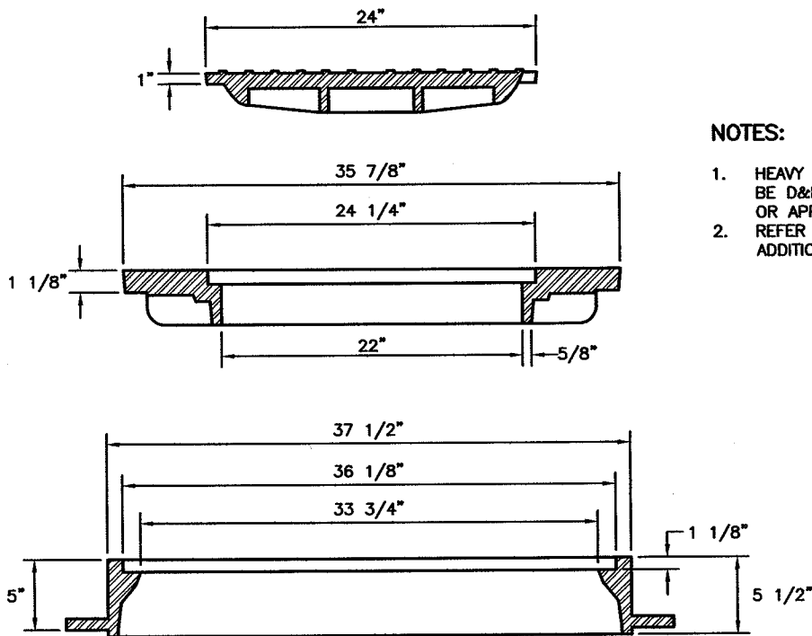
SECTION MANHOLE FRAME AND COVER
