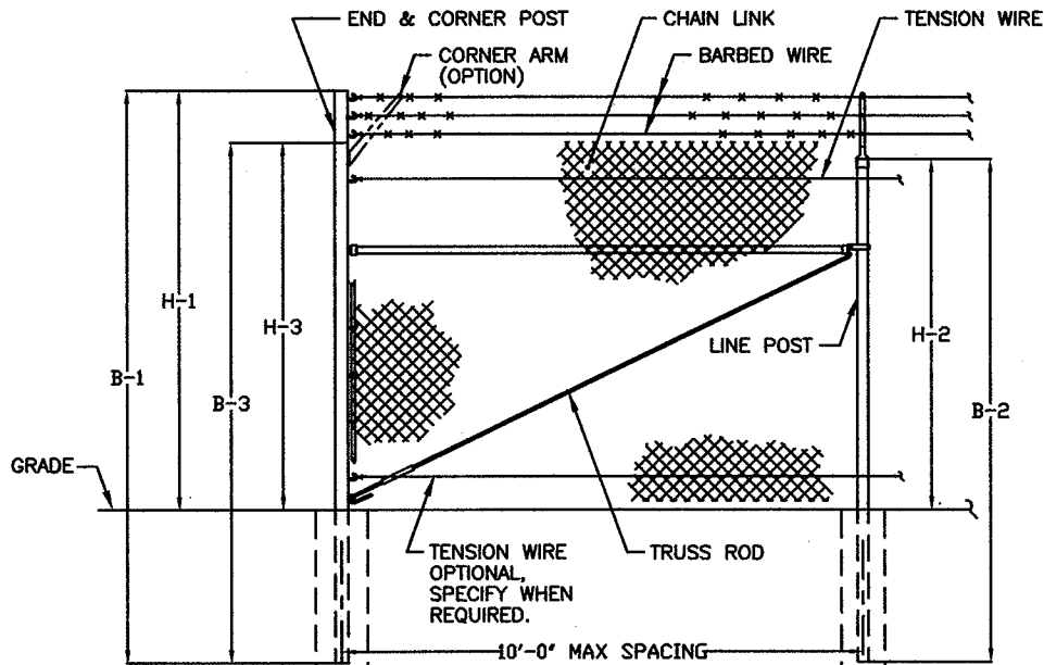
FENCE SECTION ELEVATION WITHOUT TOP RAIL & WITH BARBED WIRE
