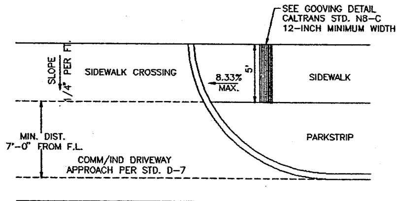
SIDEWALK NOT ADJACENT TO CURB
