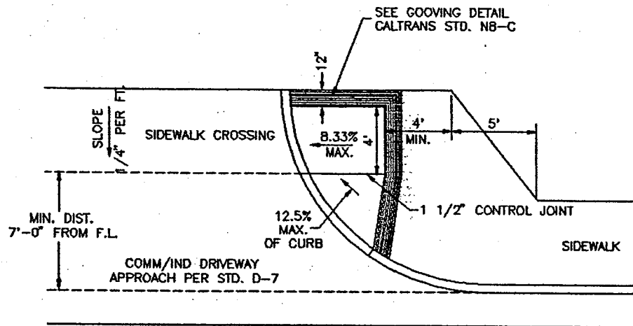
SIDEWALK ADJACENT TO CURB
