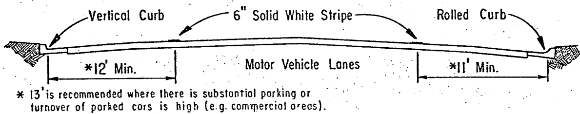
(B) PARKING PERMITTED WITHOUT PARKING STRIPE OR STALL
